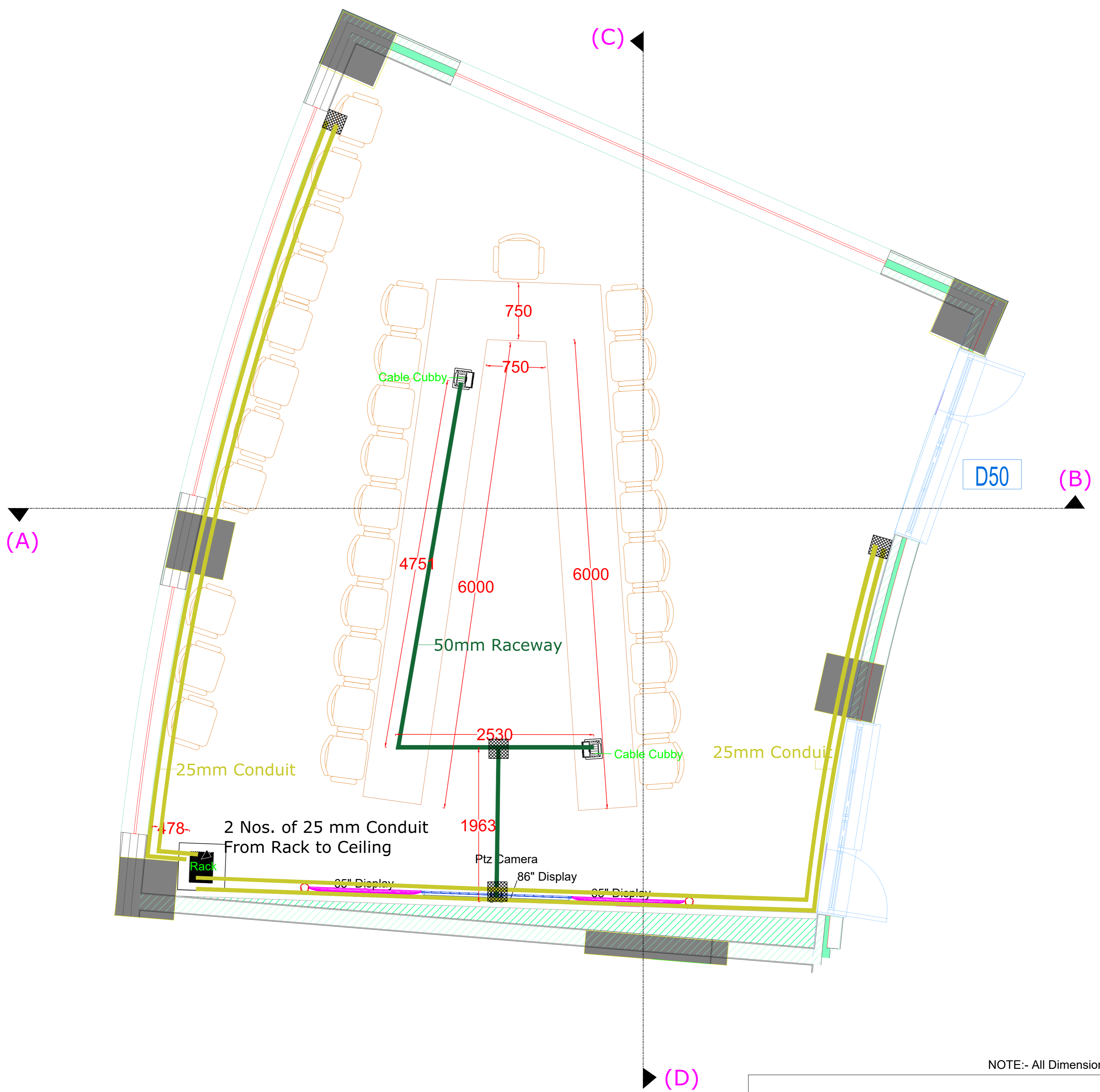
Floor Plan
