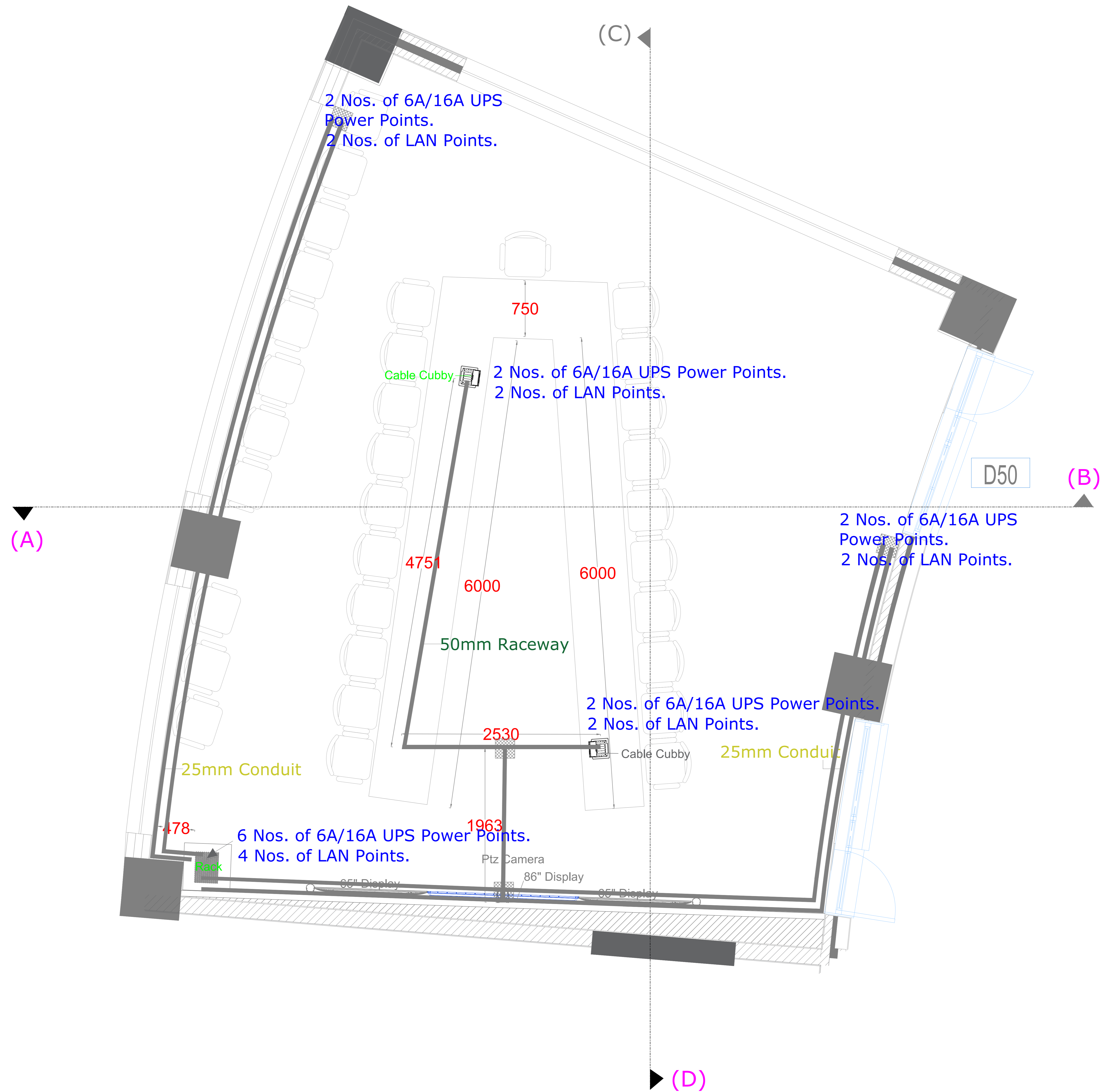
Floor Plan
