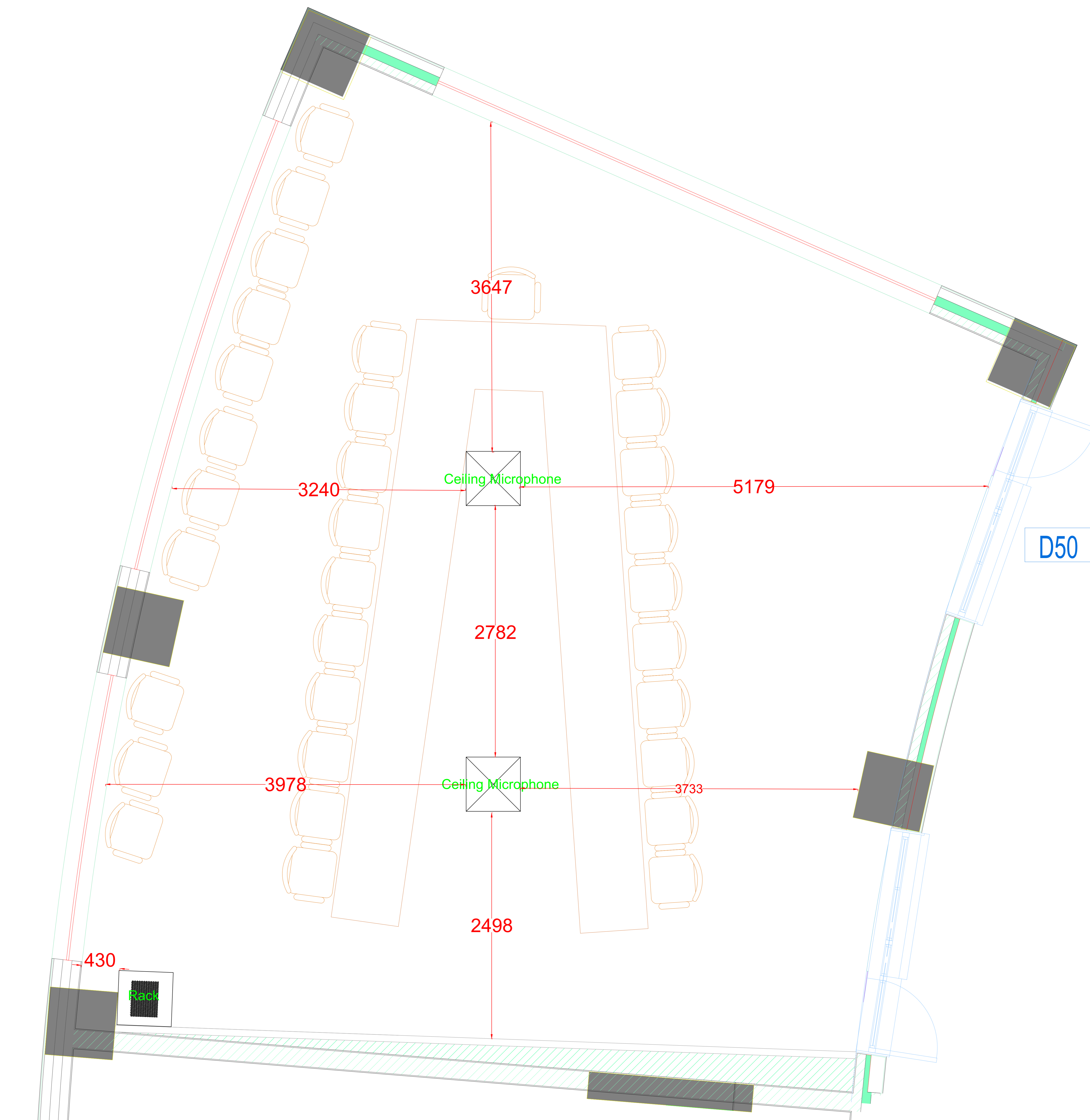
Ceiling Plan
